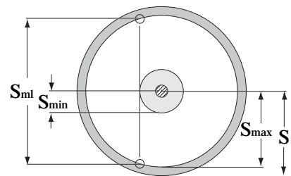
Recommended operational area for shaft displacement
